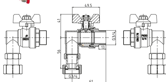
PHA-040_3 DN20
