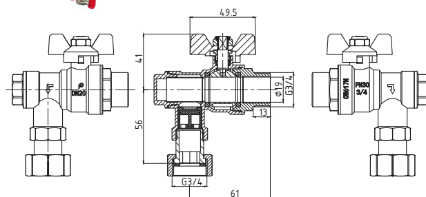
PHA-040_4 DN20
